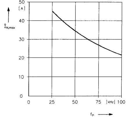
Fig.8: Dependency of the maximum allowable amplitude of the mains current \hat{I}_{N,\max} on the switching frequency f_P for application of the power module.
