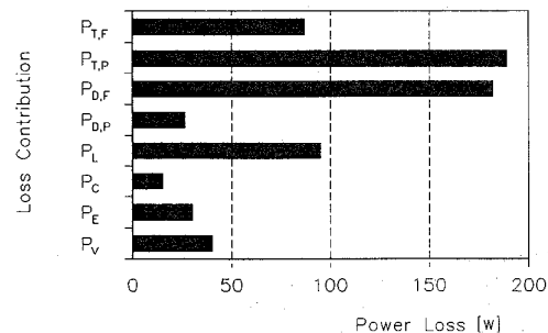
Fig.9: Graphical representation of the loss contributions of the components of a rectifier system realized with the power module IXYS VUM25-E. Operating parameters: f_P = 50 kHz, U_{N, \text{rms}} = 230 V, U_O = 700 V, T_s = 75^\circ\text{C} ; P_O \approx 16 kW, \eta = 0.96 .
