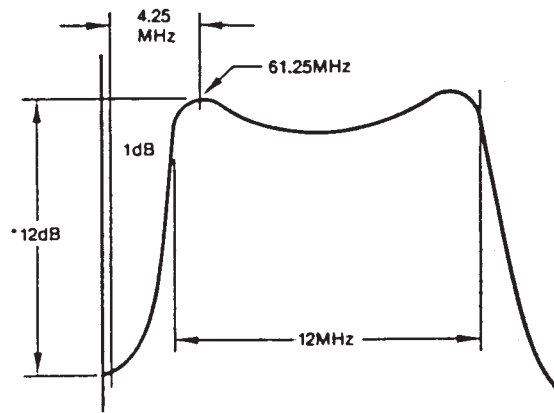
TYPICAL BANDPASS FILTER RESPONSE
