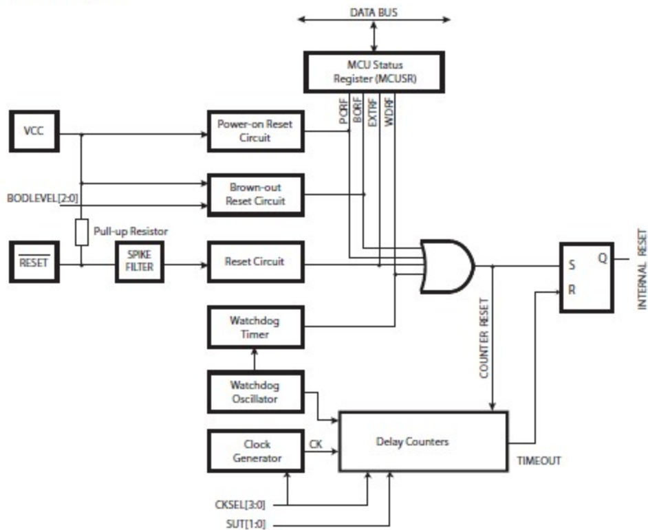
Figure 8-1. Reset Logic
