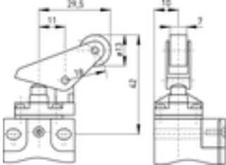
Metall-Parallelhebel WPHM
