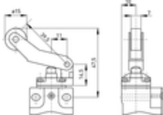
Langer Metall-Rollenhebel WHLM
