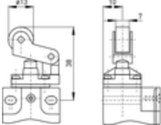
Metall-Rollenhebel WHM
