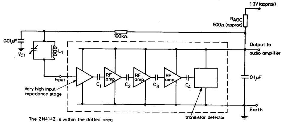
ZN414Z System Diagram
