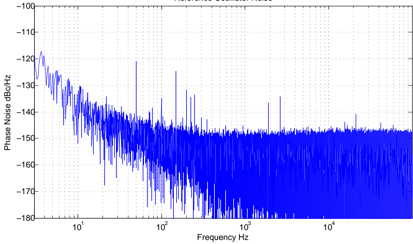
Reference Oscillator Noise
