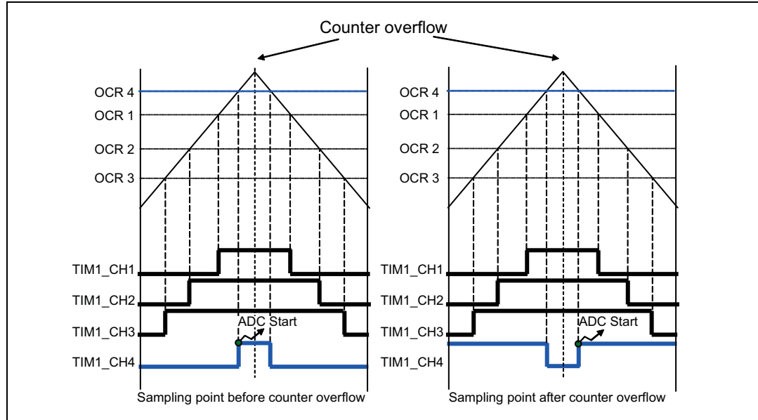
Figure 23. PWM and ADC synchronization
