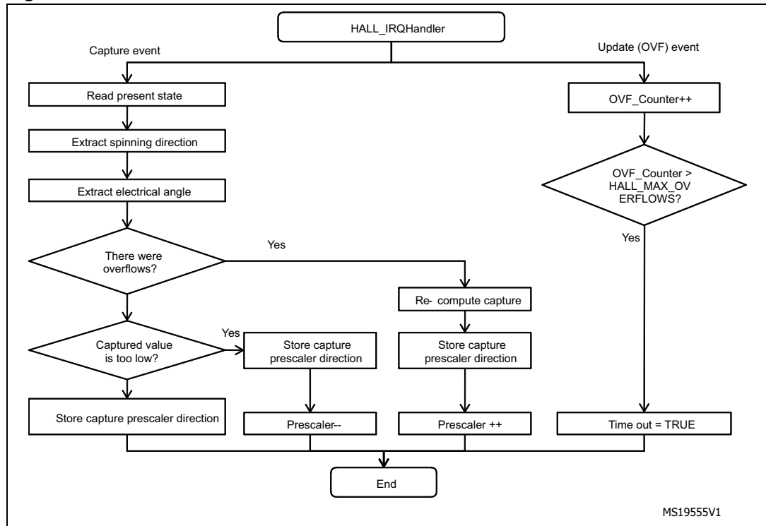
Figure 46. TIMx_IRQHandler flowchart
