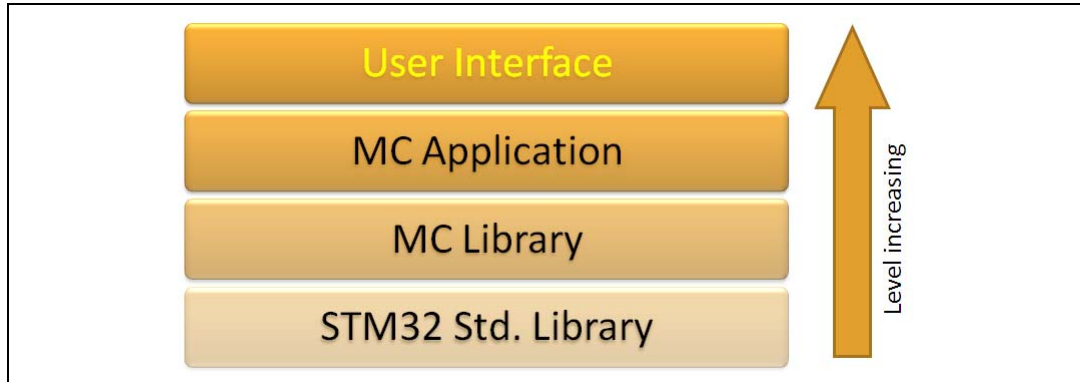
Figure 73. Software layers
