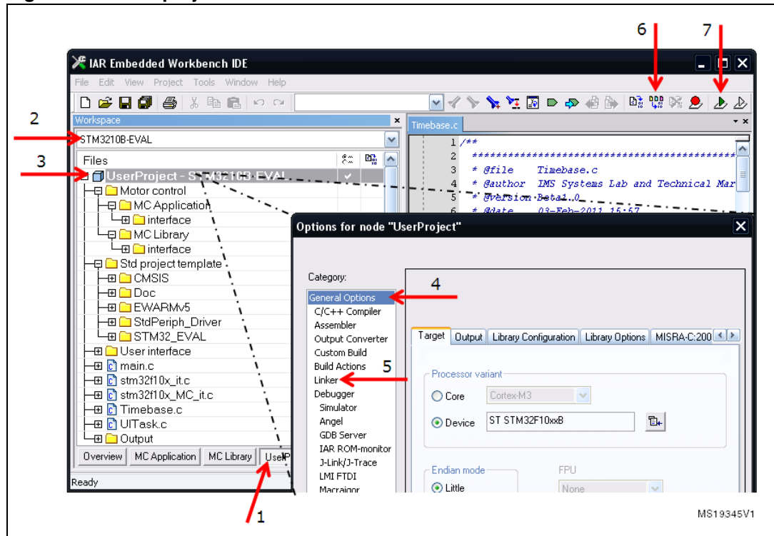
Figure 56. User project
