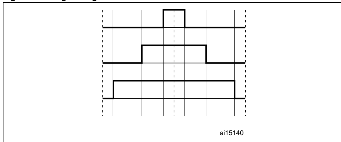
Figure 35. Regular region
