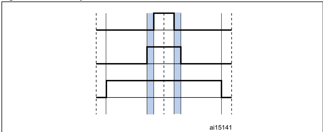
Figure 36. Boundary 1
