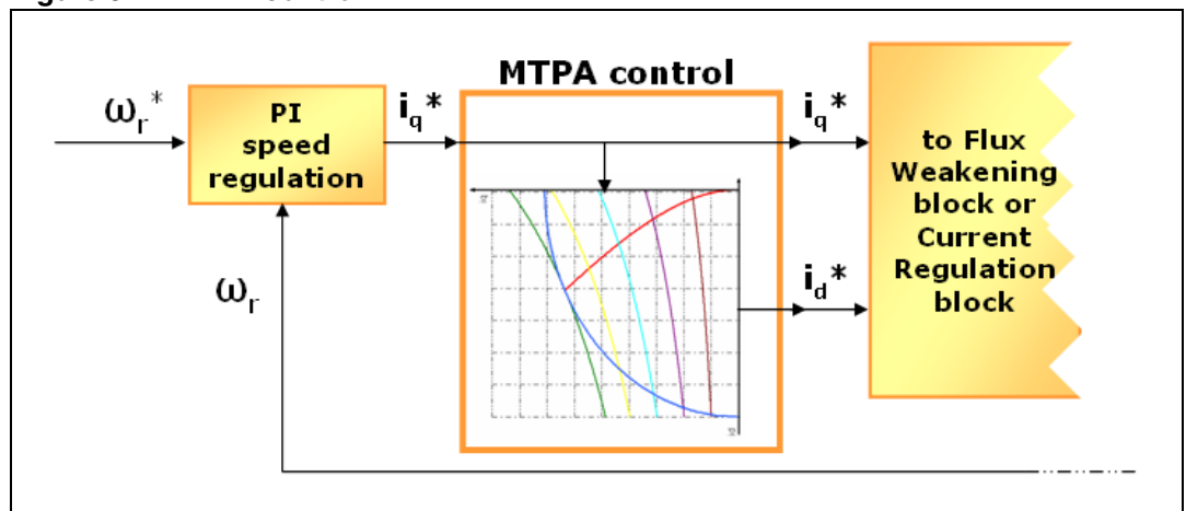
Figure 9. MTPA control
