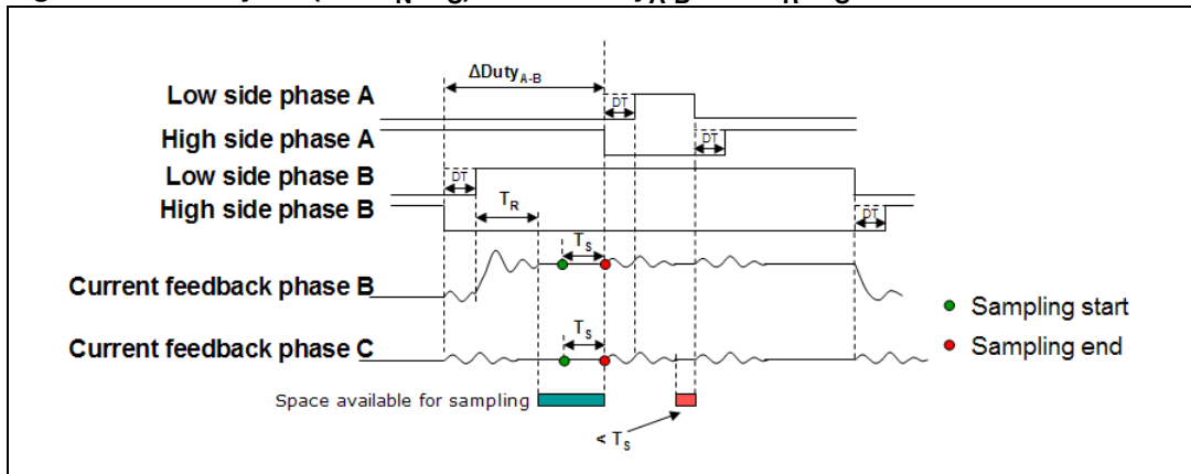
Case 4: \Delta\text{Duty}_A < (\text{DT} + \text{T}_N + \text{T}_S)/2 and \Delta\text{Duty}_{A-B} < \text{DT} + \text{T}_R + \text{T}_S
