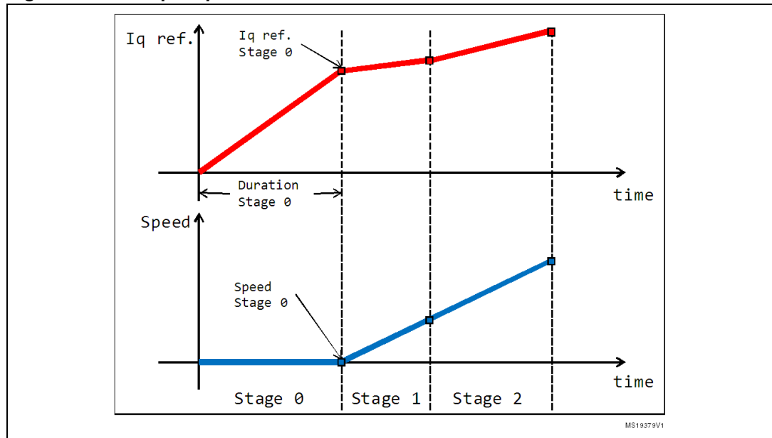
Figure 86. Revup sequence
