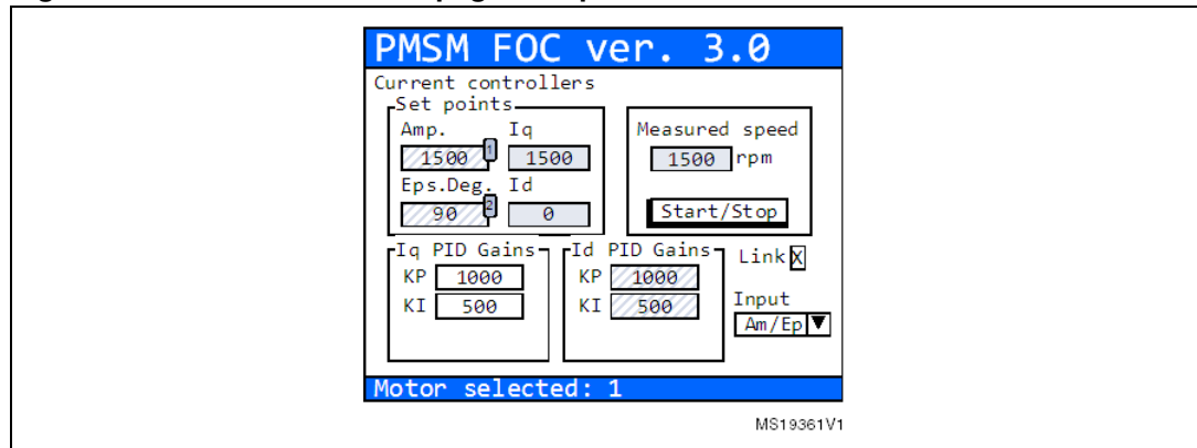
Figure 68. Current controller page with polar coordinates
