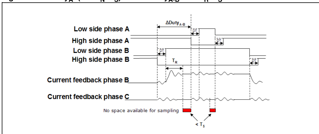
Figure 29. \Delta\text{Duty}_A < (\text{DT} + \text{T}_N + \text{T}_S)/2 and \Delta\text{Duty}_{A-B} < \text{DT} + \text{T}_R + \text{T}_S
