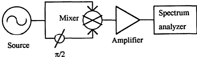
Fig. 5. Block diagram of system used to measure the PM noise of the mixers at 10.6 GHz and 21.2 GHz.
