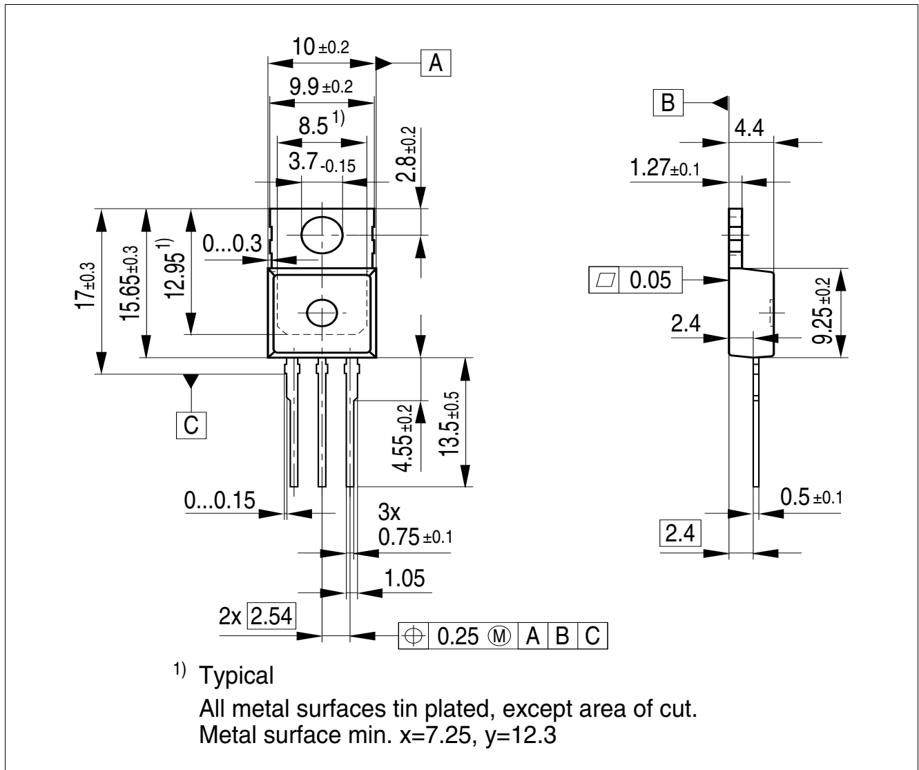
Figure 1 PG-TO220-3-1
