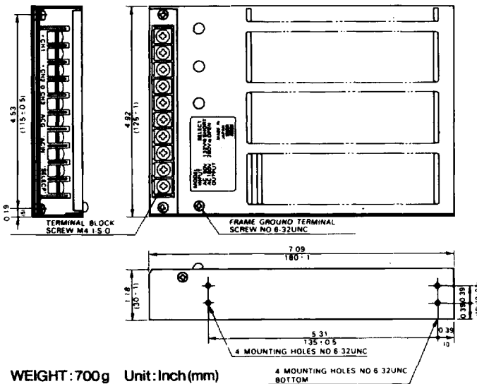
WEIGHT: 700g Unit: Inch(mm)
