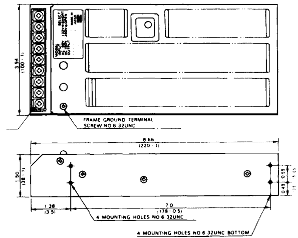
WEIGHT: 740g Unit: Inch(mm)
