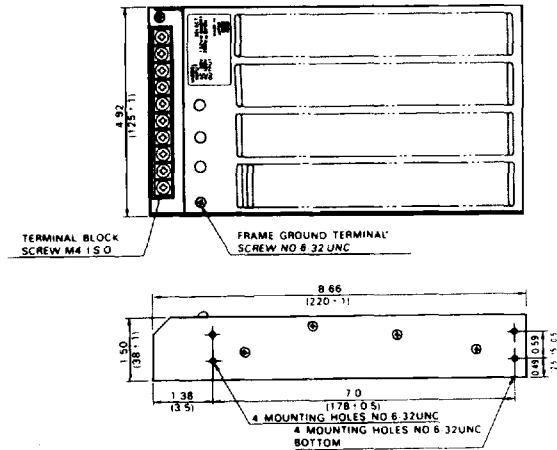
WEIGHT: 890g Unit: Inch(mm)
