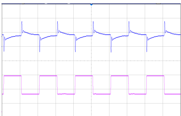
Figure 4 Dynamic response for 25% load step (25% ~ 50% ~ 25%) and 0.1A/ \mu\text{s} slew rate, (2ms/div), see Figure 10 for test configuration; CH1-output voltage (200mV/div); CH2-output current (2.5A/div)
