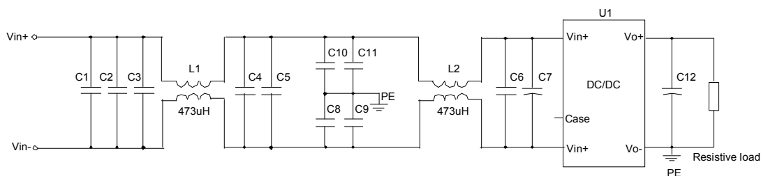
Figure 16 EMC test configuration
