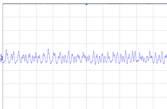
Figure 3 Input reflected ripple current (2 \mu\text{s}/\text{div} , 50mA/div), see Figure 15 for test configuration
