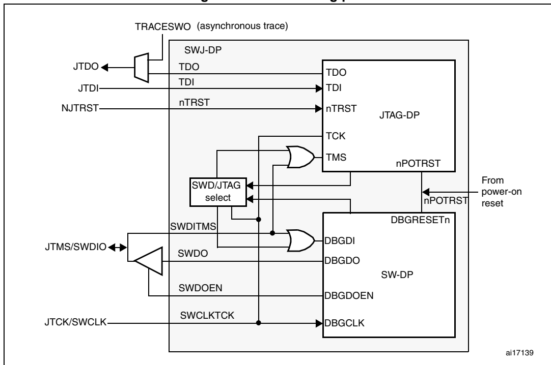
Figure 484 shows that the asynchronous TRACE output (TRACESWO) is multiplexed with TDO. This means that the asynchronous trace can only be used with SW-DP, not JTAG-DP.
