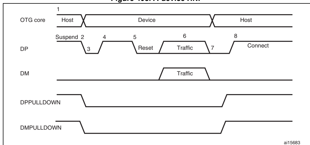
Figure 408. A-device HNP
