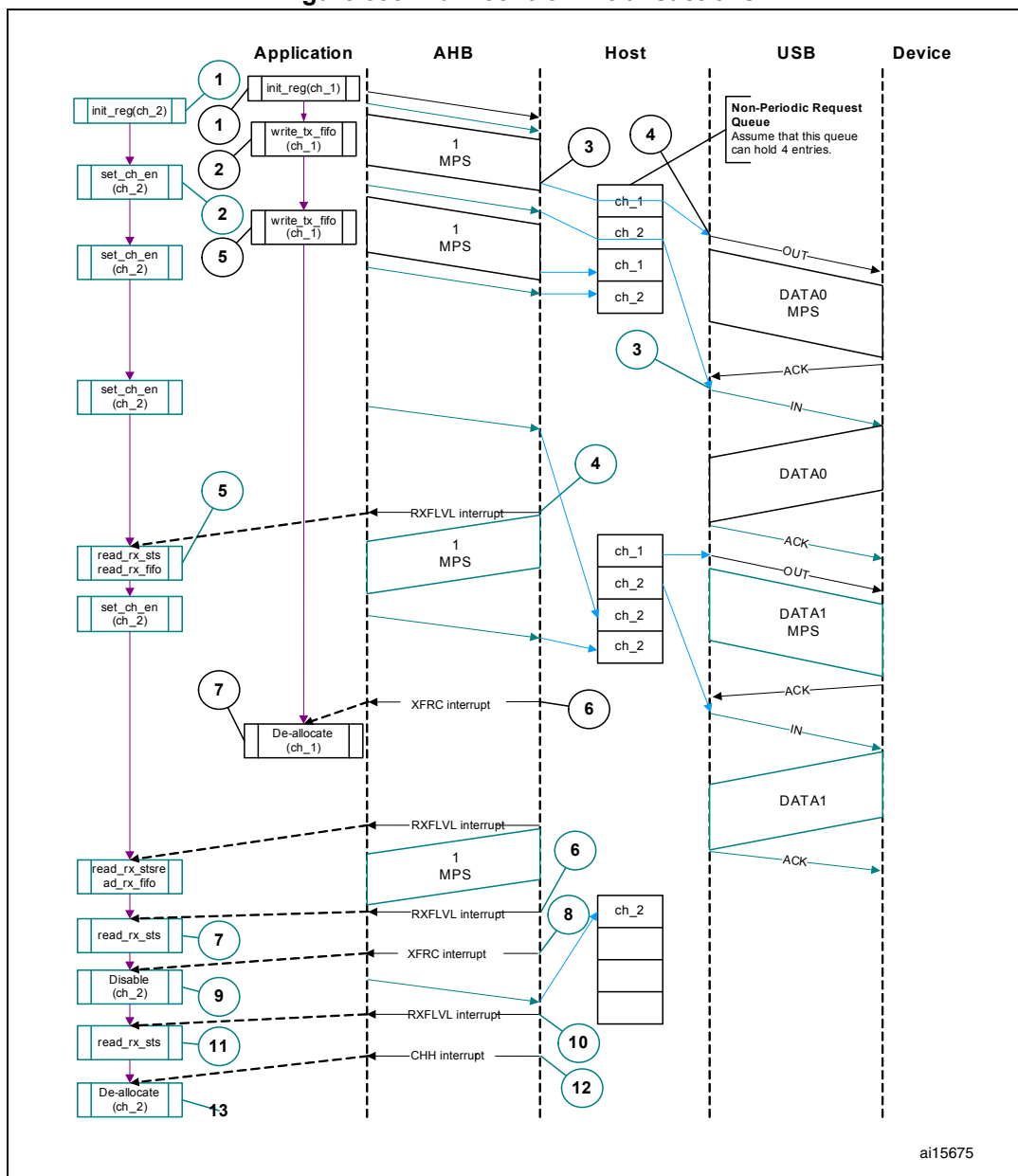
Figure 399. Bulk/control IN transactions
