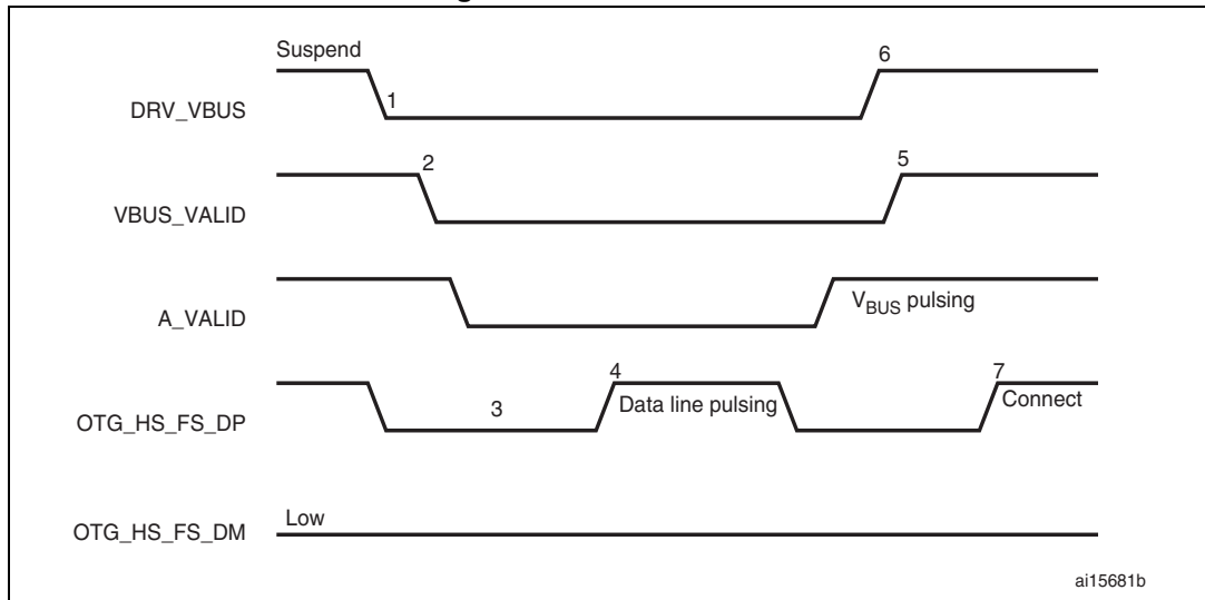
Figure 428. A-device SRP
