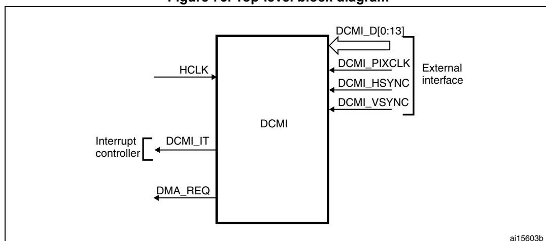
Figure 73. Top-level block diagram
