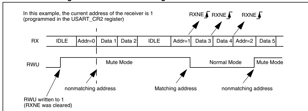
Figure 304. Mute mode using address mark detection
