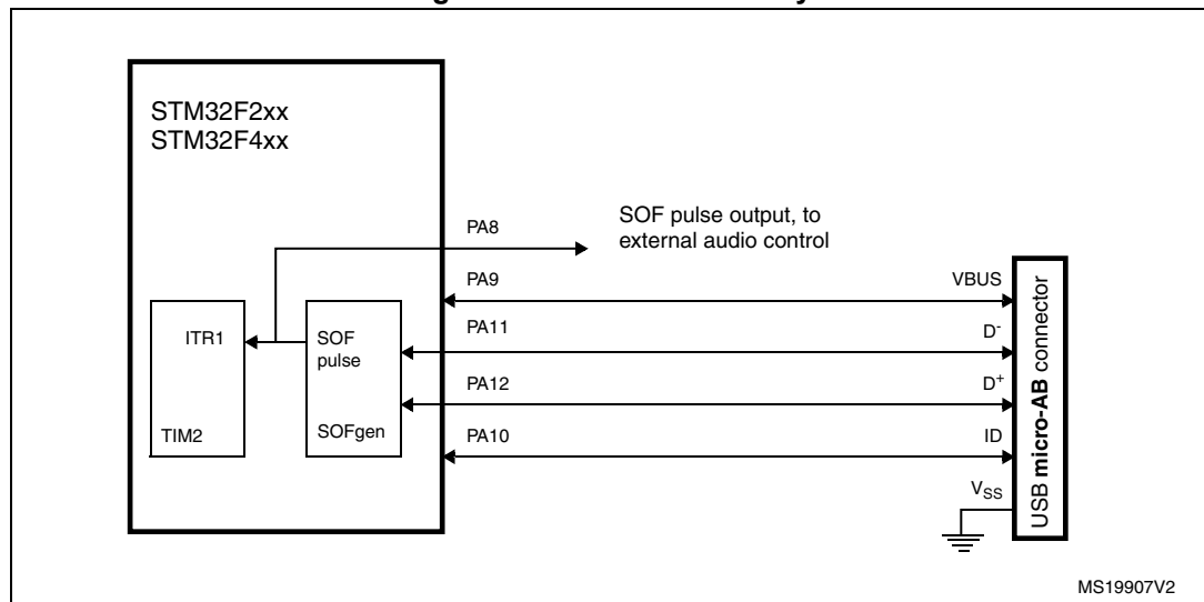
Figure 390. SOF connectivity
