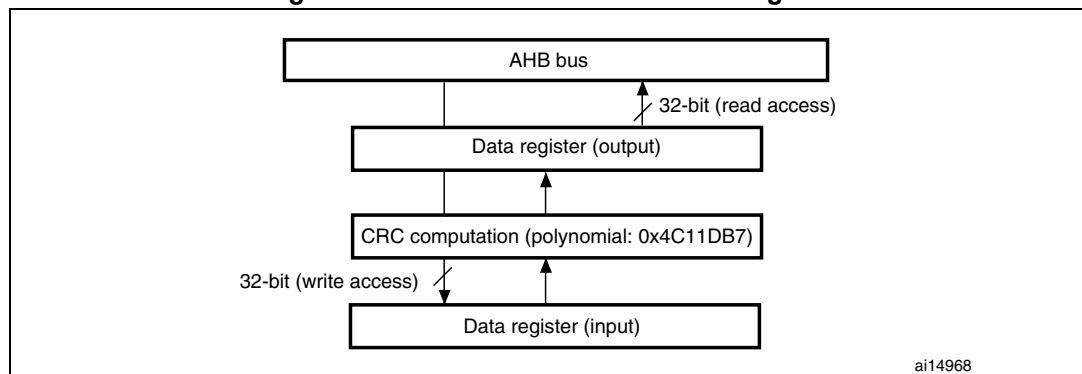
Figure 8. CRC calculation unit block diagram
