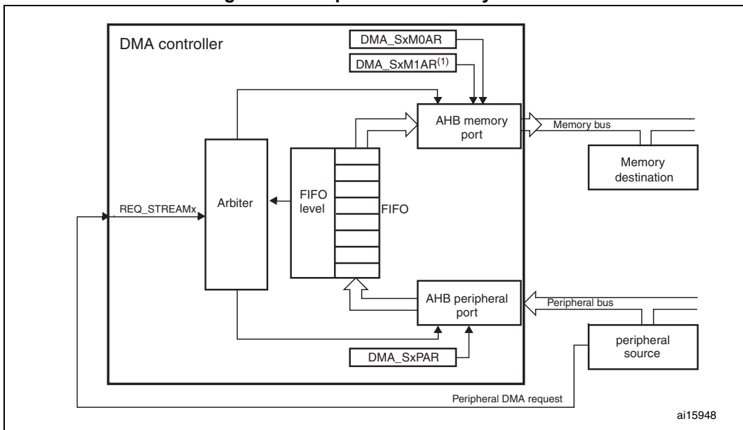
Figure 36. Peripheral-to-memory mode
