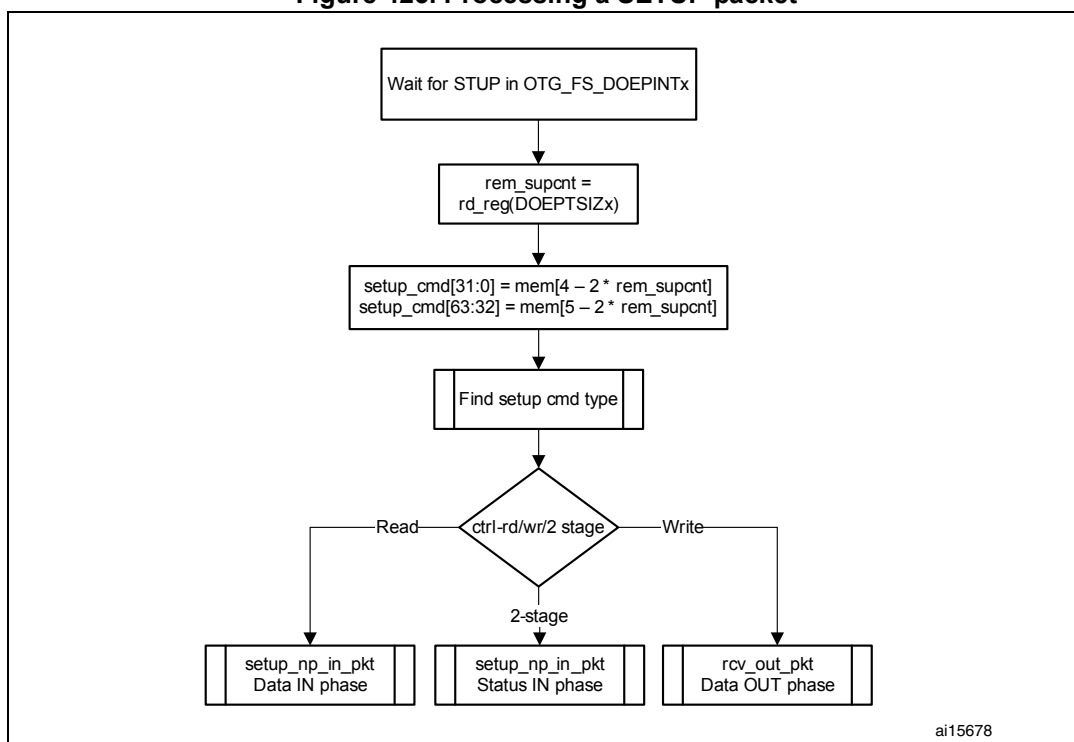
Figure 425. Processing a SETUP packet
