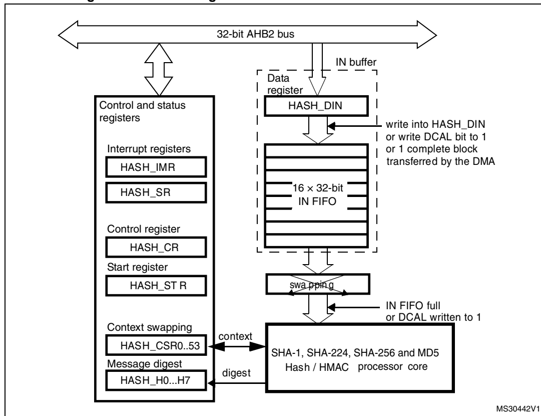
Figure 234. Block diagram for STM32F42xxx and STM32F43xxx
