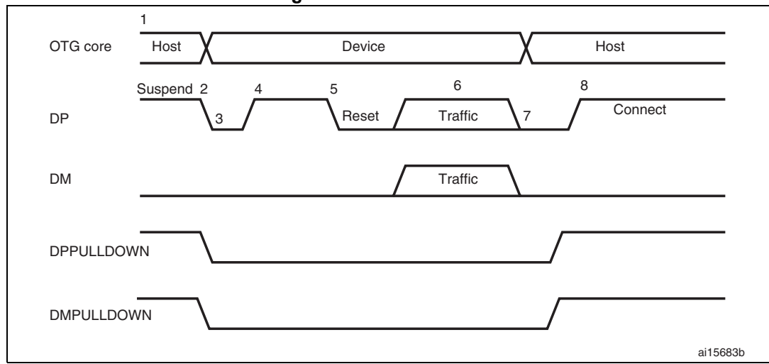
Figure 430. A-device HNP
