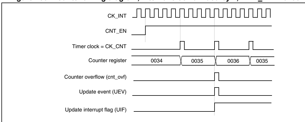
Figure 150. Counter timing diagram, internal clock divided by 4, TIMx_ARR=0x36
