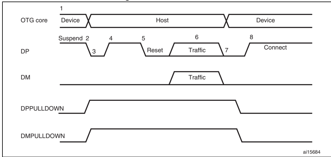
Figure 409. B-device HNP
