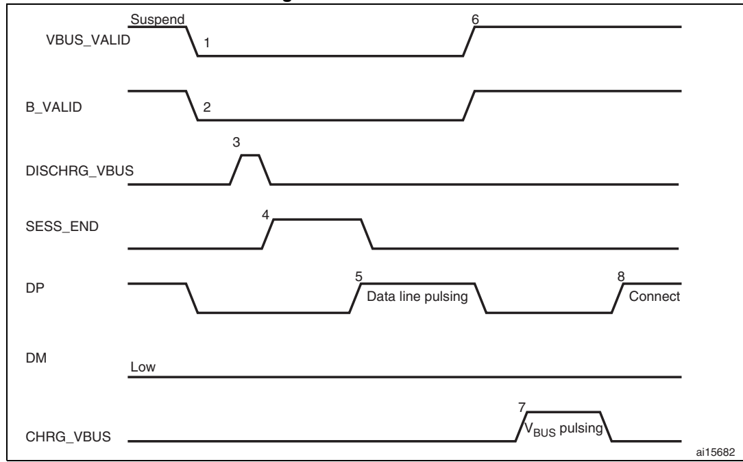
Figure 407. B-device SRP
