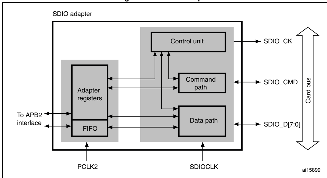
Figure 327. SDIO adapter
