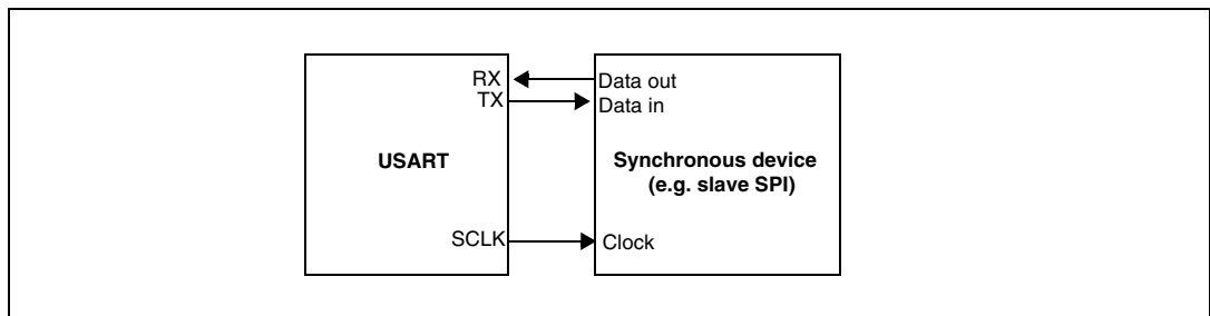
Figure 307. USART example of synchronous transmission
