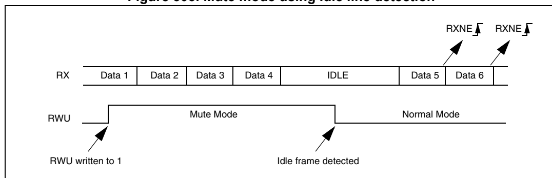
Figure 303. Mute mode using Idle line detection
