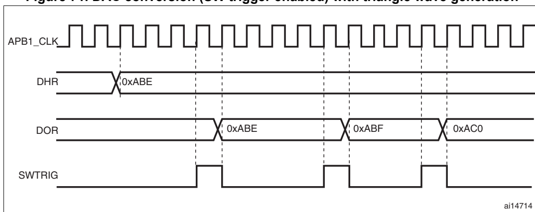
Figure 71. DAC conversion (SW trigger enabled) with triangle wave generation
