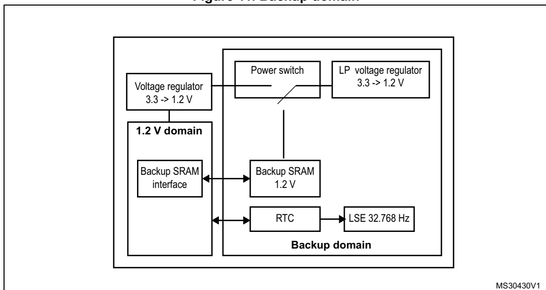
Figure 11. Backup domain
