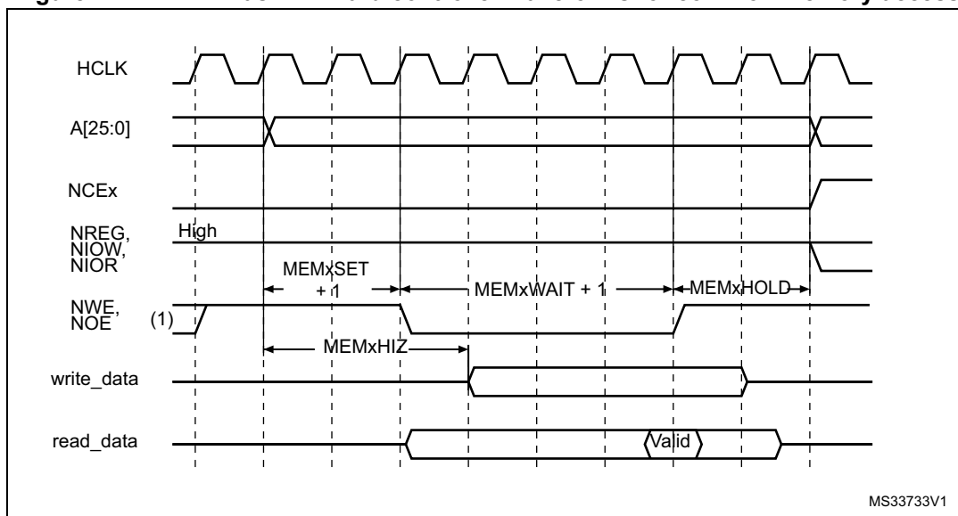
Figure 474. NAND Flash/PC Card controller waveforms for common memory access
