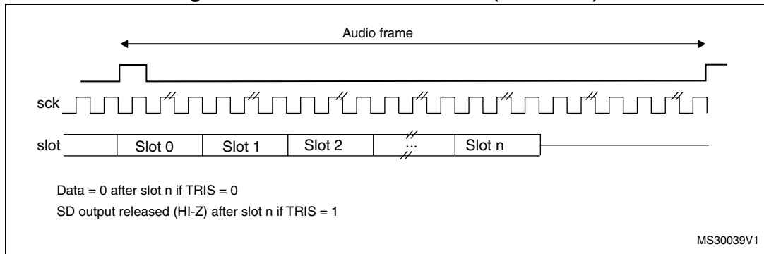
Figure 286. FS role is start of frame (FSDEF = 0)
