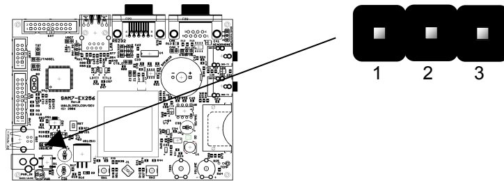
Figure 10-16 – USB/EXT Configuration
