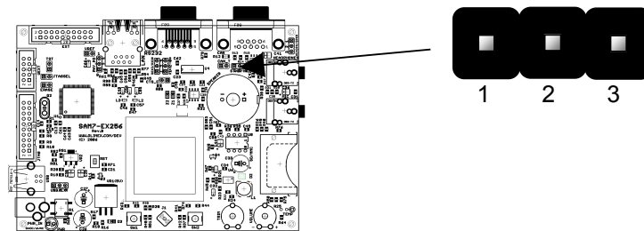
Figure 10-21 - STNB/HS Configuration
