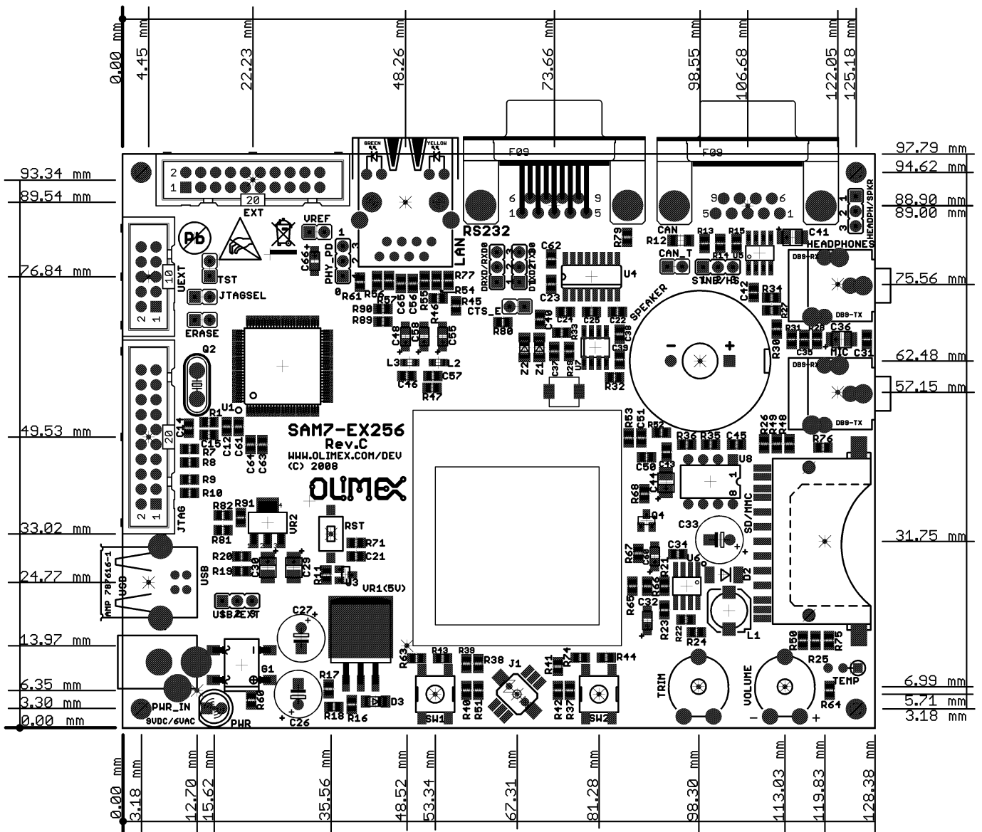
Figure 13-30. Mechanical Drawing
