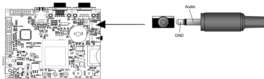
Figure 9-12 - Headphone Connector
