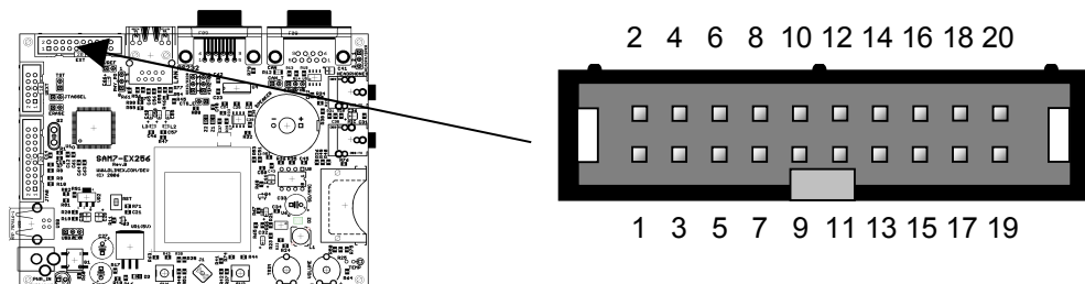
Figure 9-13 - EXT Connector
