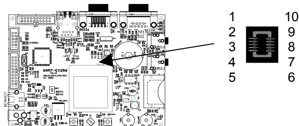
Figure 9-5 - LCD Connector
