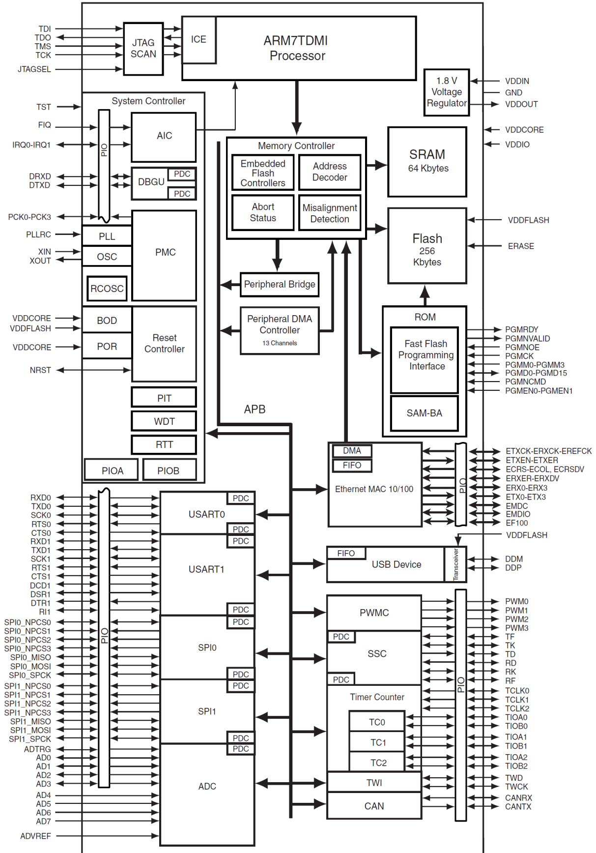
Figure 4-3. Block Diagram
