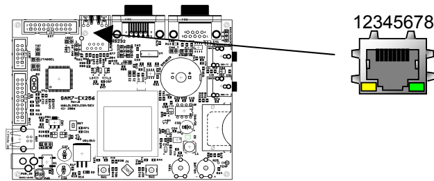
Figure 9-6 - Ethernet Connector
