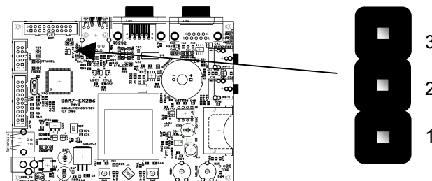
Figure 10-17 – PHY_PD Configuration
