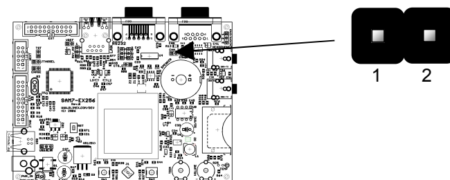
Figure 10-22 - CAN_T Configuration
