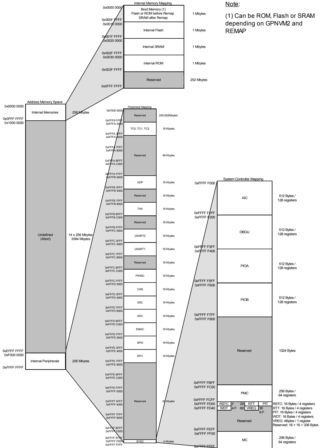
Figure 11-28 - Memory Map
