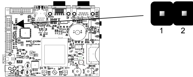
Figure 10-25 - JTAGSEL Configuration
