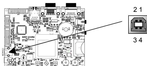
Figure 9-7 - USB Connector
