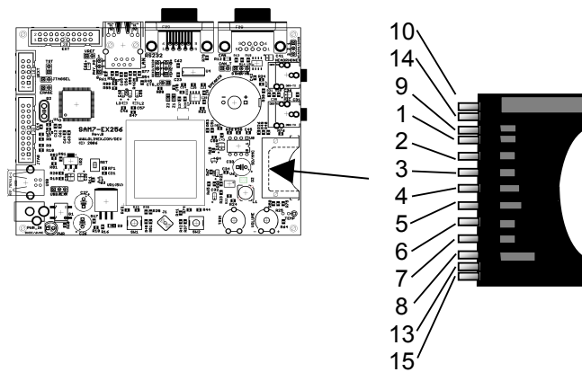
Figure 9-8 - SD/MMC Connector
