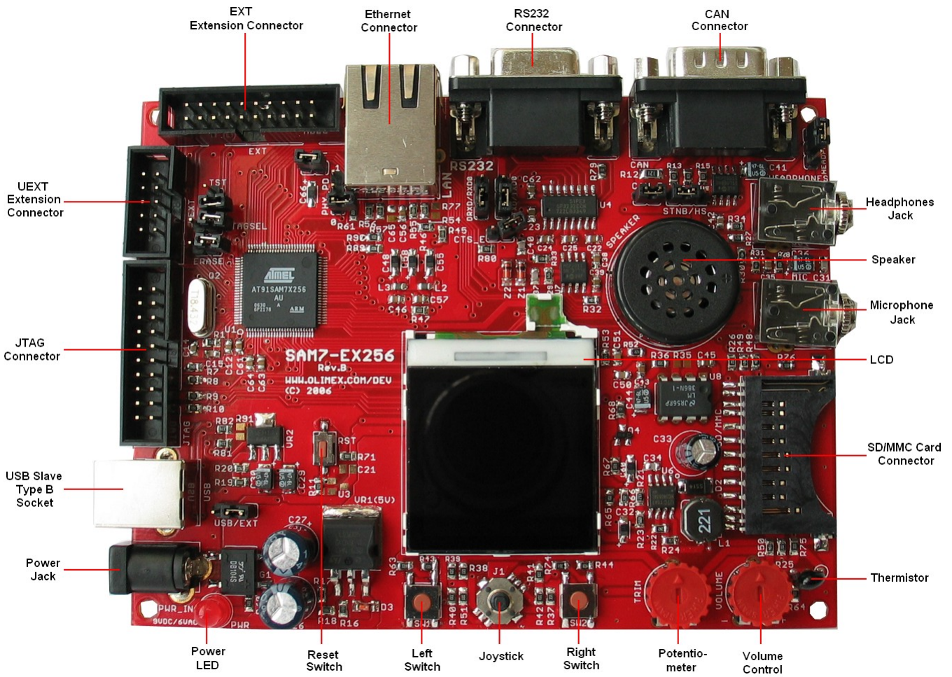
Figure 3-2. Board Layout
