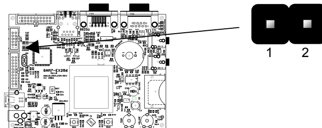
Figure 10-26 - ERASE Configuration
