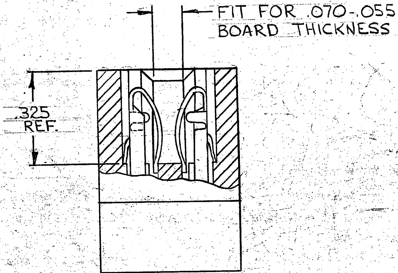
SECTION A-A SCALE - 5-1 CONTACT SHOWN FOR REF. ONLY.
