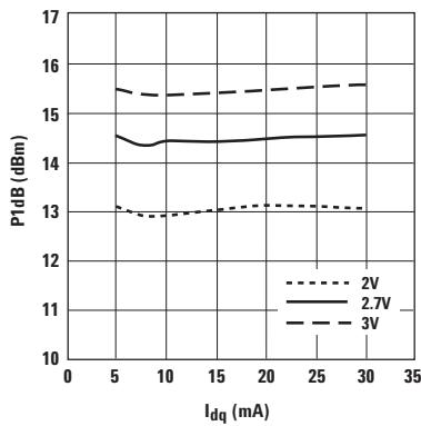
Figure 15. P1dB vs. I_{dq} and V_{ds} at 2 GHz. [1,2]
