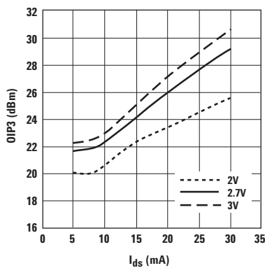
Figure 18. OIP3 vs. I_{ds} and V_{ds} at 900 MHz. [1]
