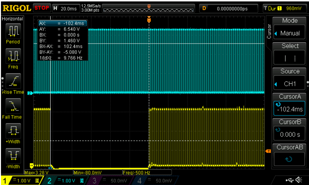
Illustration 1: Measured run-time of the ESP8266WiFiMult::run() function (blue channel Interrupt input, yellow channel LED output)
