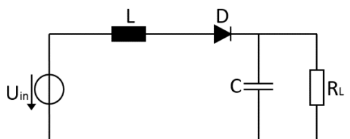
Fig. 9. Boost converter circuit in state of low gate (PWM) signal.
