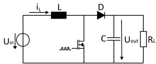
Fig. 7. Boost converter circuit.
