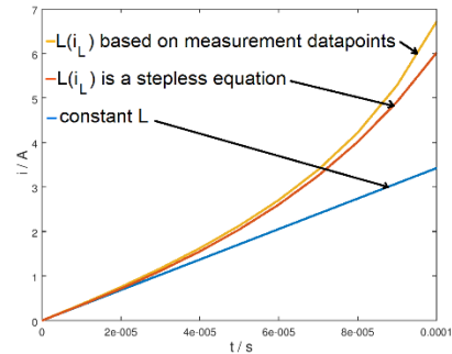
Fig. 4. Inductor current traces modeled with and without saturation.
