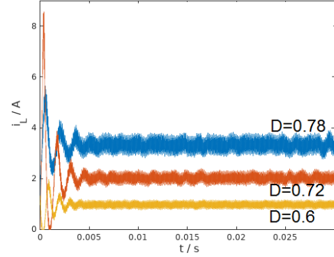
Fig. 11. Time traces of the inductor current for different duty cycles.
