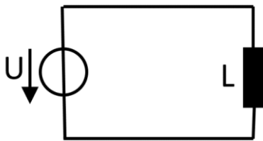
Fig. 3. Test circuit for a transient simulation of saturation.
