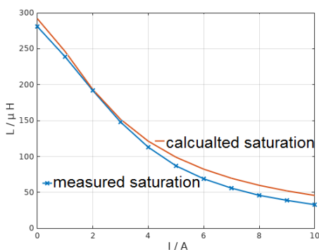
Fig. 6. Calculated and measured saturation - Core 77310-A7, N=57 turns.
