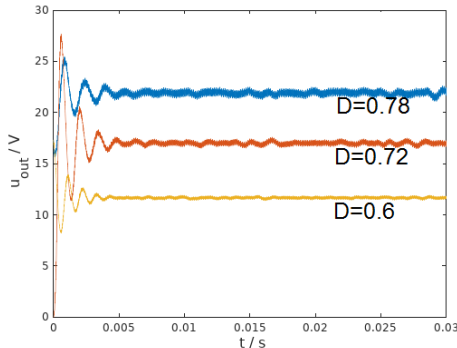
Fig. 10. Time traces of the output voltage for different duty cycles.
