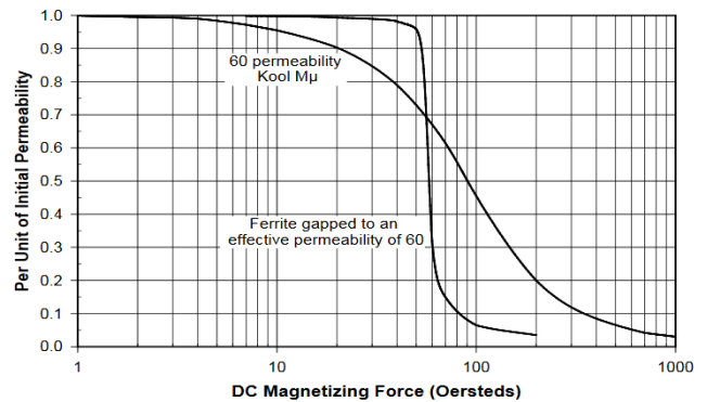
Fig. 1. Saturation curve of a gapped ferrite and a powder core with the same effective permeability [6].
