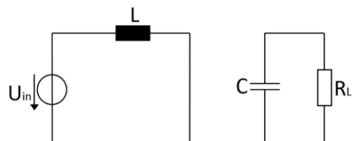
Fig. 8. Boost converter circuit in state of high gate (PWM) signal.
