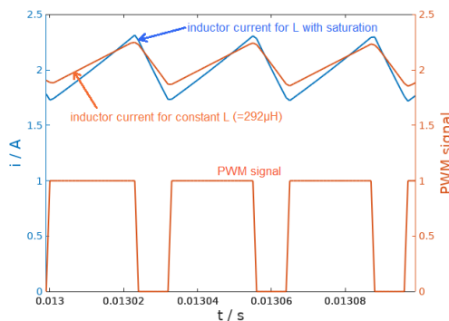
Fig. 12. Boost converter simulation results with and without considering choke saturation.
