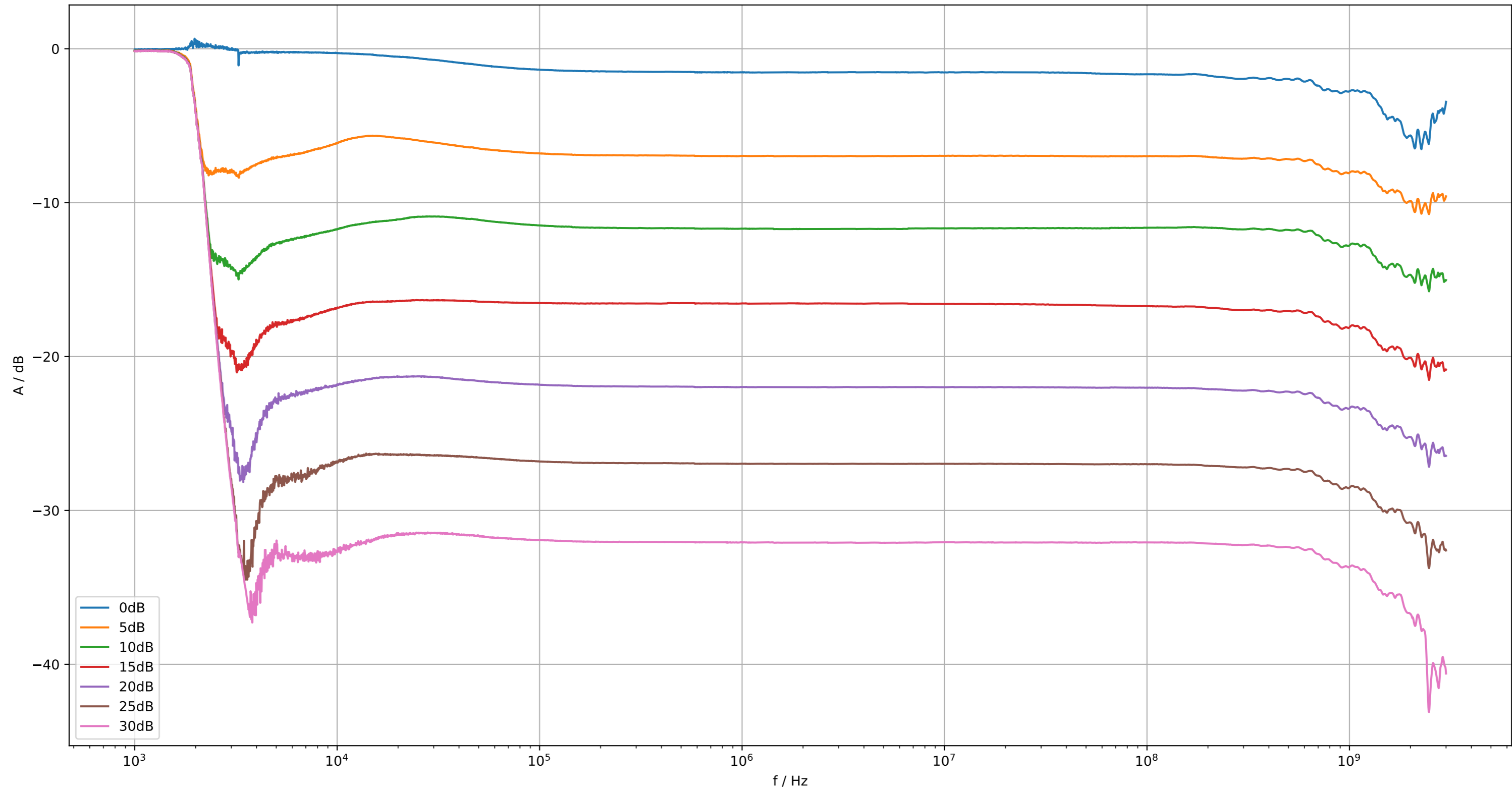
ATT-6000 30dB, Insertion Loss
