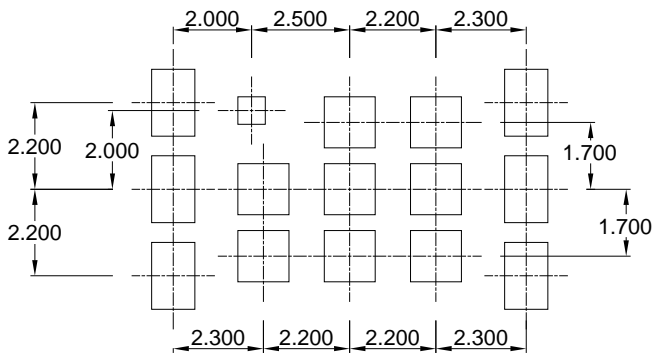
Figure A.26.2(a) LA-outline substrate/PCB layout
