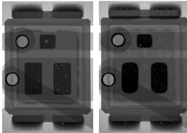
Figure 19 X-rays of DirectFET (left) and DirectFET PbF
