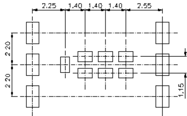
Figure A.27.3(a) L6-outline stencil design
