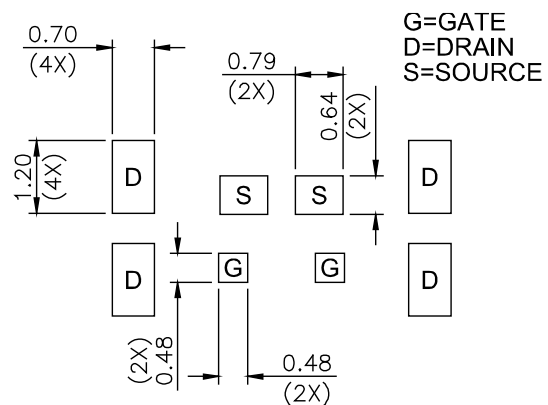
Figure A.7.3(b) SA-outline stencil design
