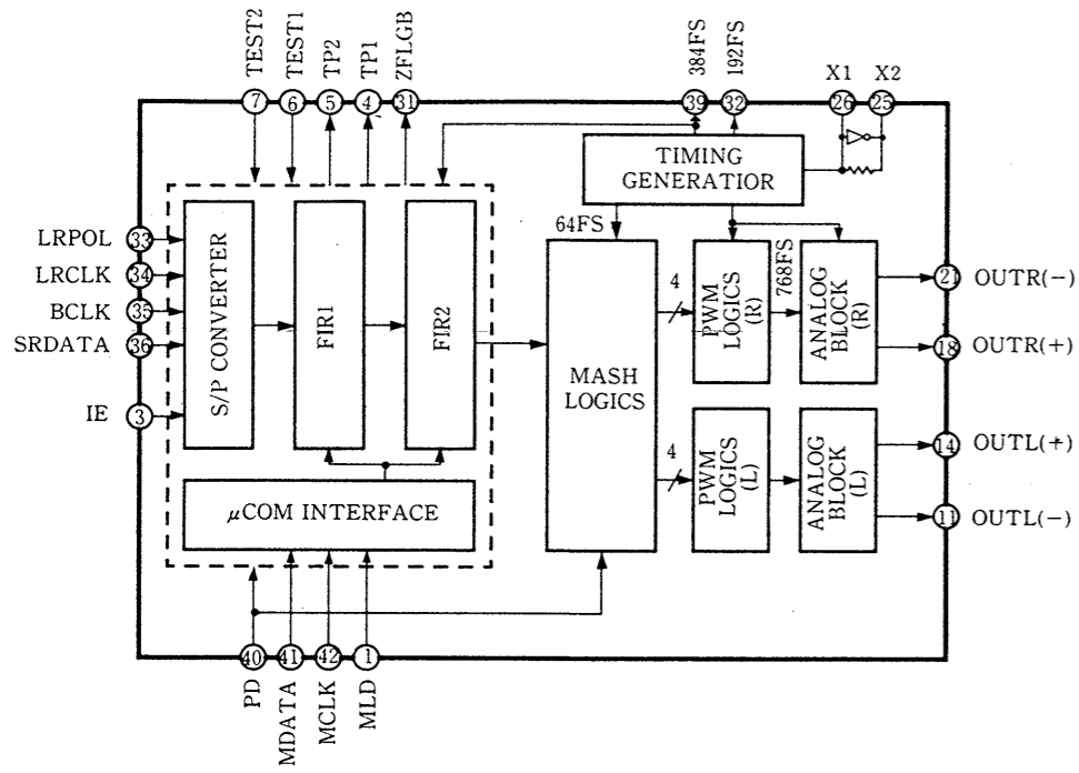
IC301 CXD8178Q
