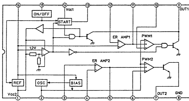
IC450 FA7616N
