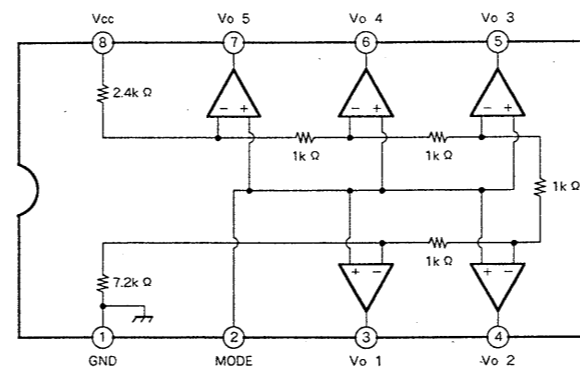
IC803 BA3818F-SY
