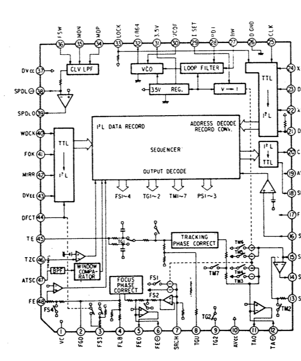
IC502 CXA1272Q
