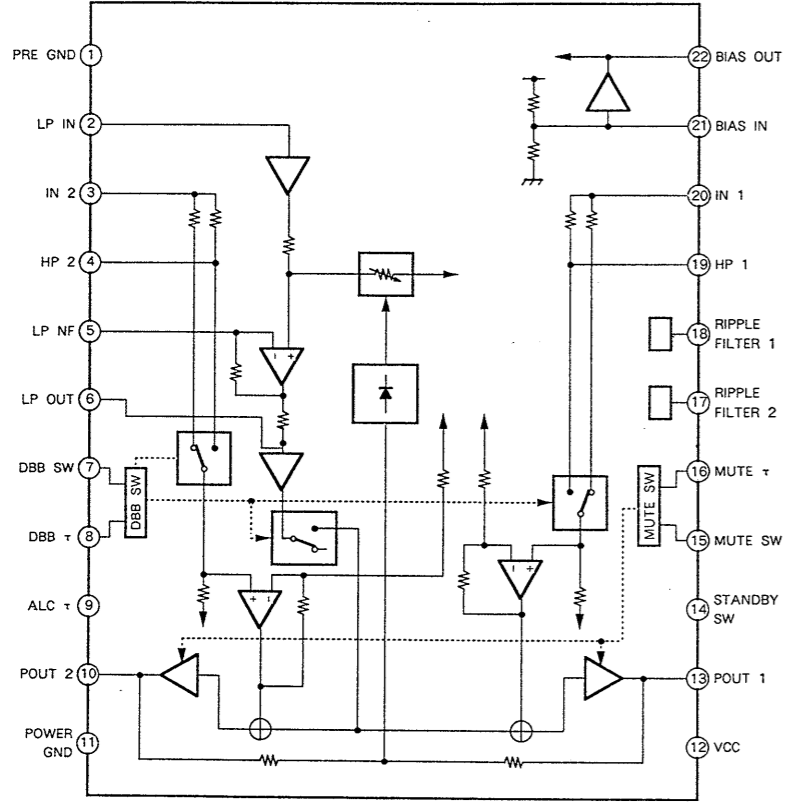
IC303 BA3570F
