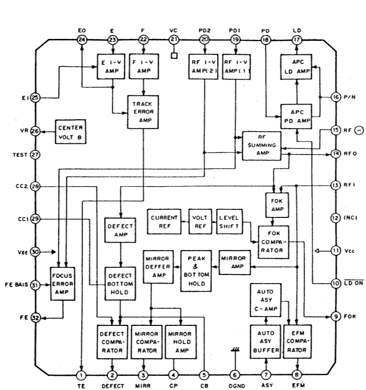
IC501 CXA1271Q
