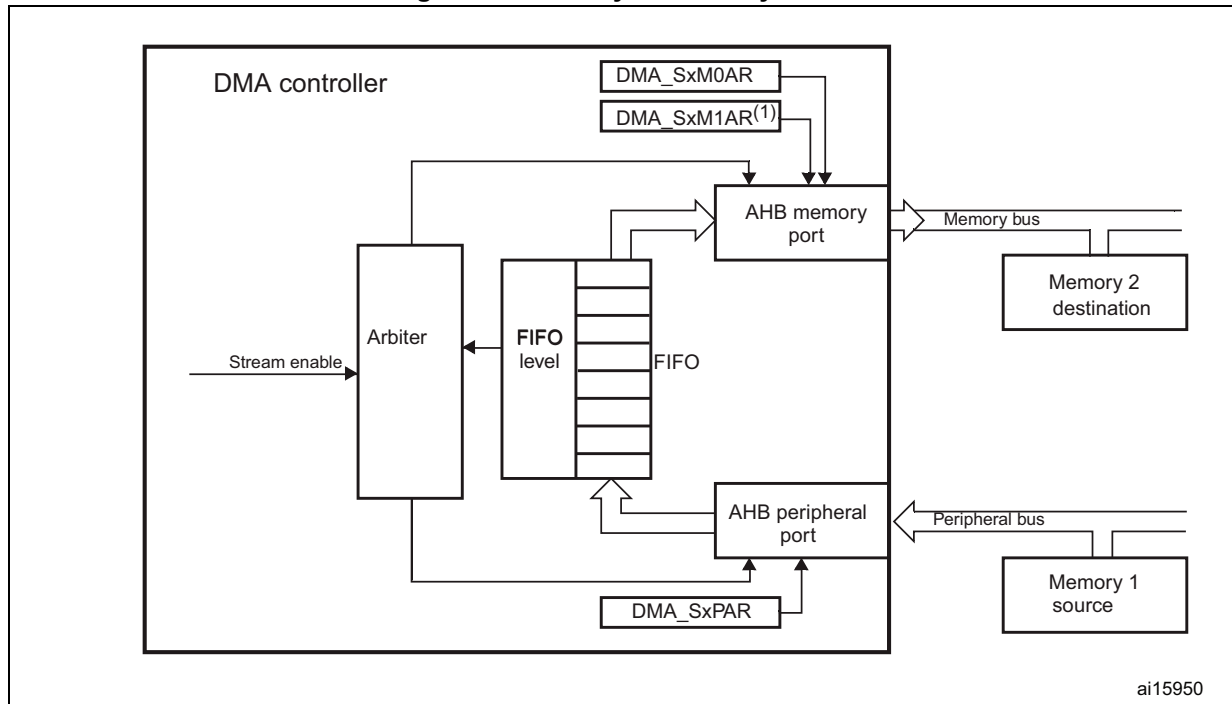
Figure 38. Memory-to-memory mode
