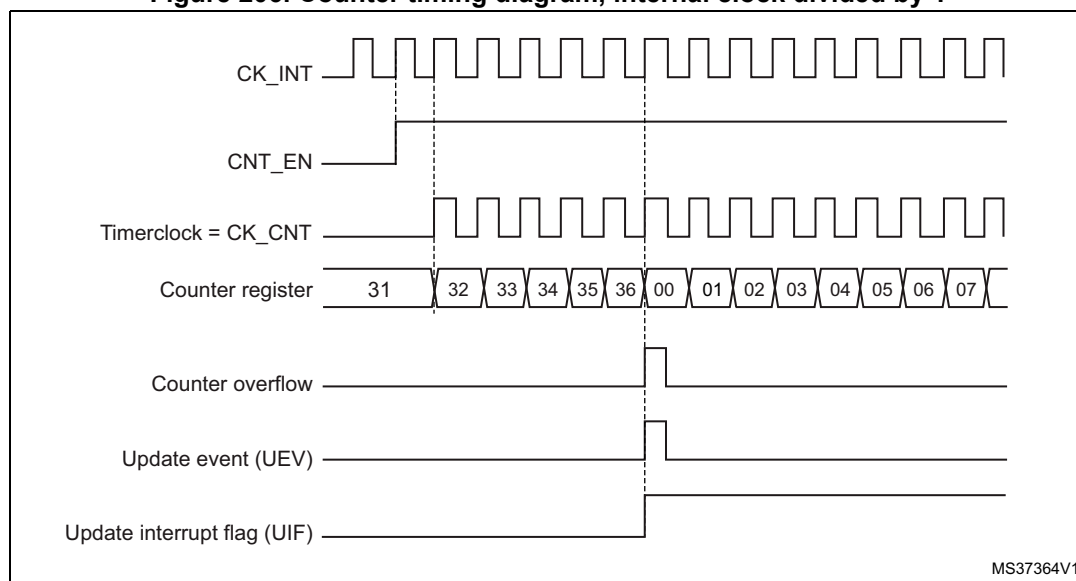
Figure 206. Counter timing diagram, internal clock divided by 1
