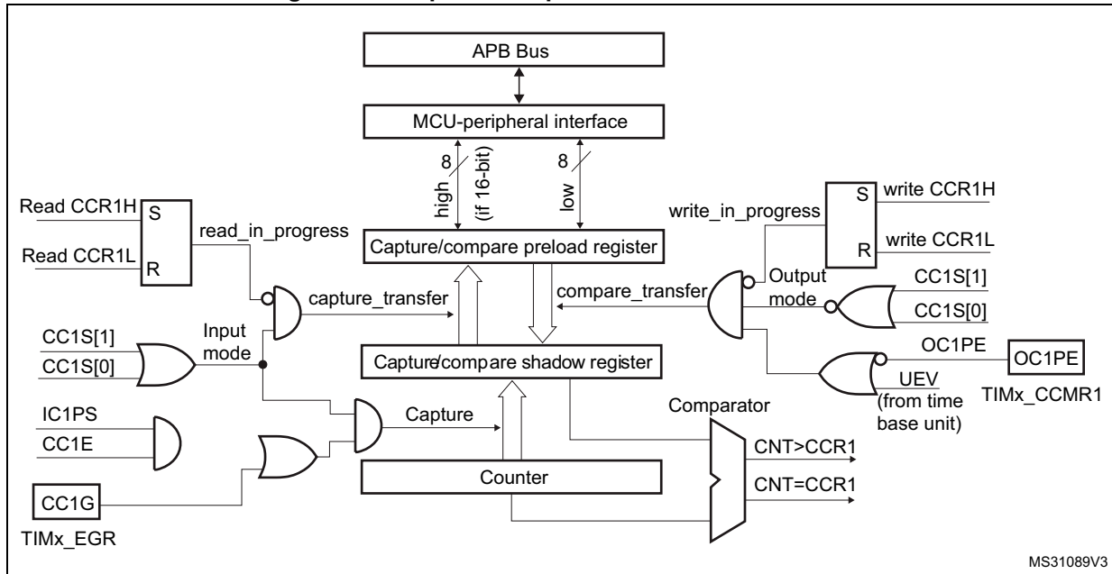
Figure 113. Capture/compare channel 1 main circuit
