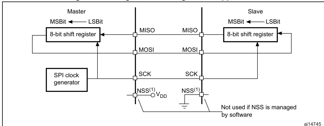
Figure 247. Single master/ single slave application
