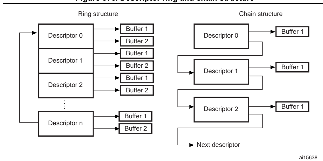
Figure 376. Descriptor ring and chain structure
