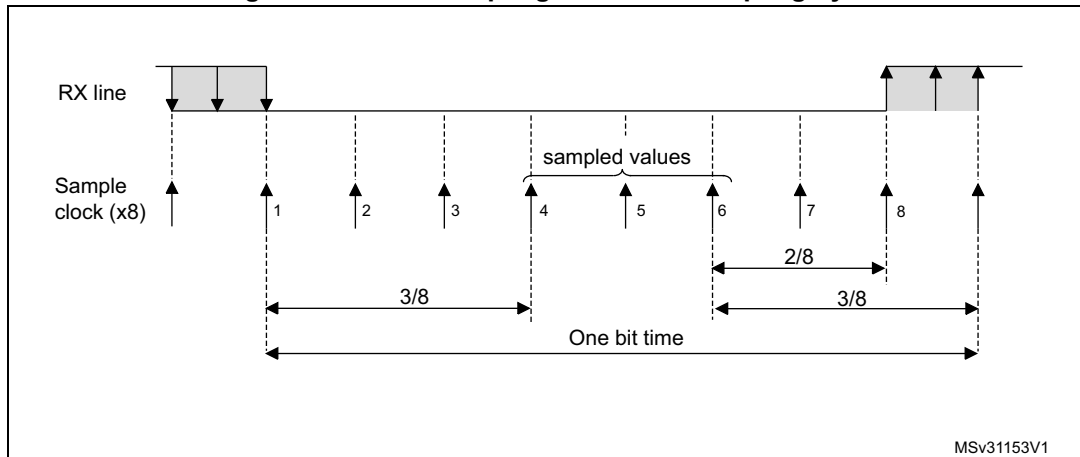
Figure 302. Data sampling when oversampling by 8
