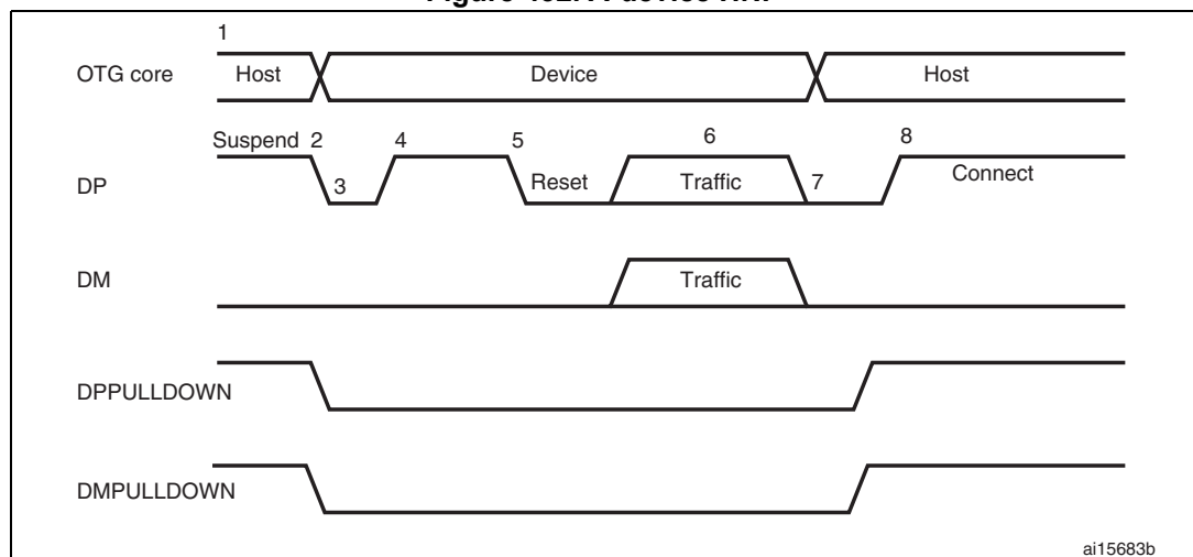
Figure 432. A-device HNP
