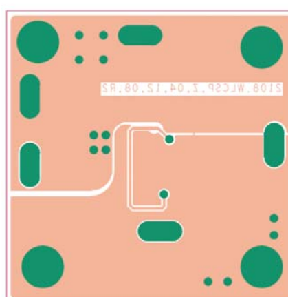
Figure 35. Recommended TSOT Bottom Layer
