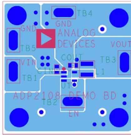
Figure 34. Recommended TSOT Top Layer
