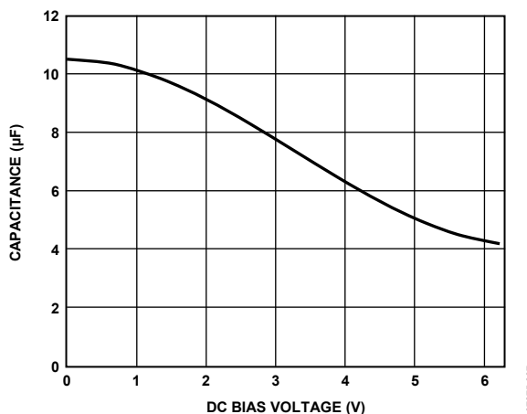
Figure 30. Typical Capacitor Performance
