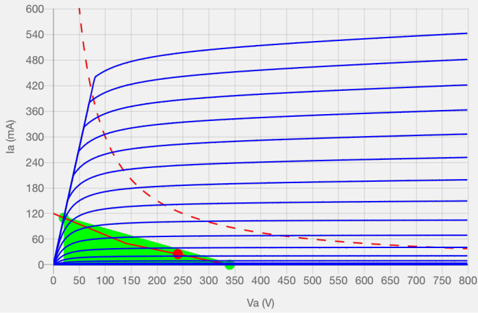
Anode Characteristic Graph: 807 - www.vtadiy.com
