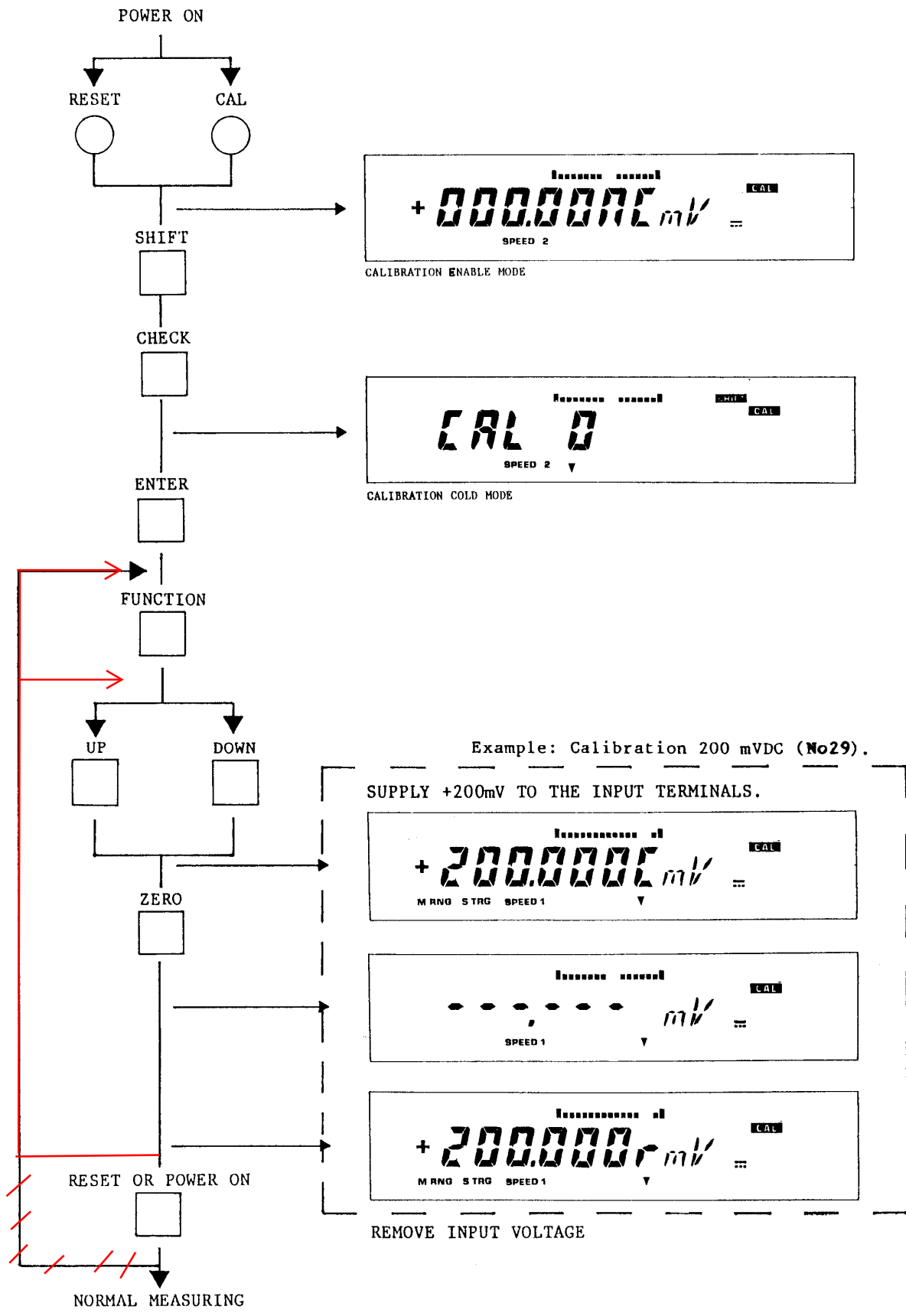
Flow-chart for electronic calibration by manual control
