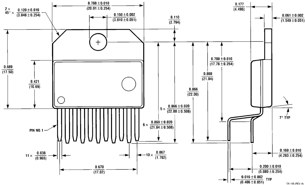
Molded TO-220 Package (TA) Order Number LM2984T NS Package Number TA11B
