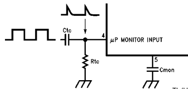
FIGURE 2. Monitoring Square Wave \mu P Signals
