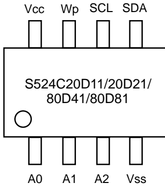
PIN CONFIGURATION
